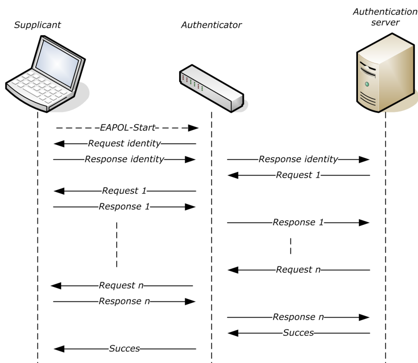
Figure 4.6: Simplified EAP authentication procedure[63]
