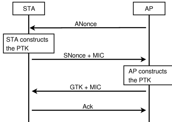
Figure 3.2: The 4-Way Handshake [62]
