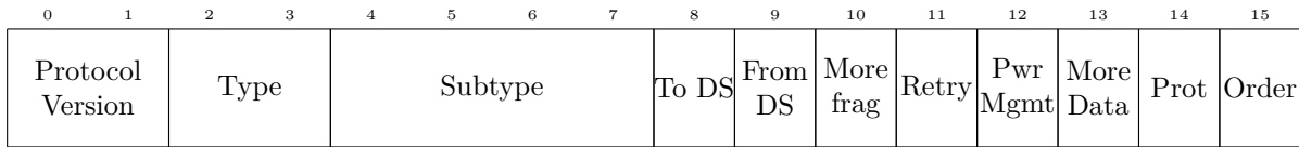
Figure 2.5: Frame Control subfields in bits
