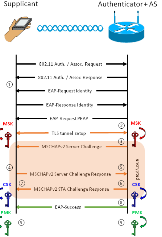
Figure 2: General PEAP authentication sequence
